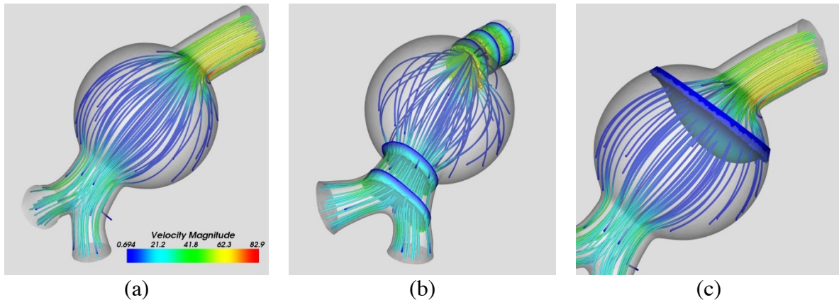
Figure 7. Details of the flow after inserting of the aneurism. Streamlines (a), streamlines and modulus of the velocity profile and a zoom in the region of the aneurism (c).
